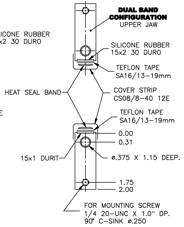
JAW BAR MACHINING (TYP. BOTH ENDS)
